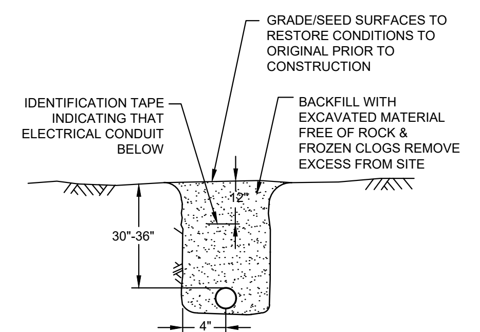
2 BURIED CONDUIT DETAIL E-501 SCALE: NONE
