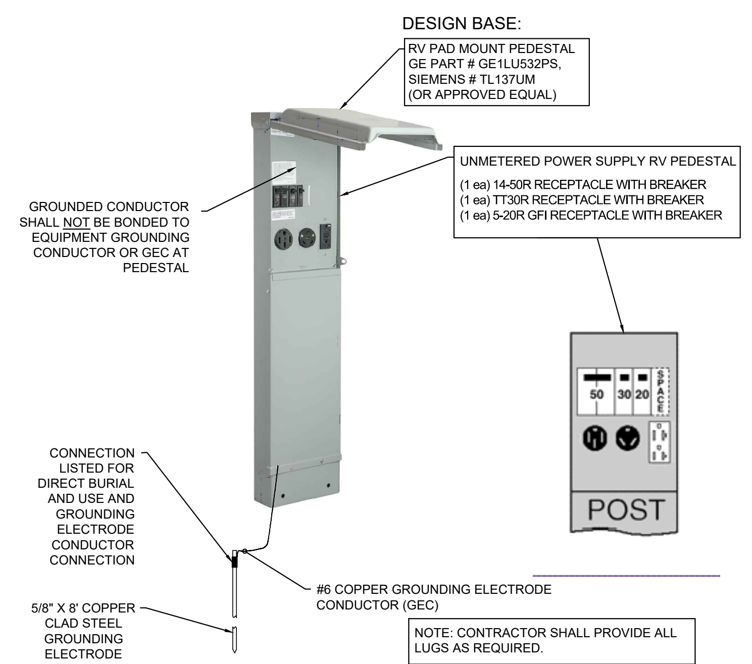
3 CAMPSITE SERVICE PEDESTAL WITH FEED-THRU LUGS E-501 SCALE: NONE
