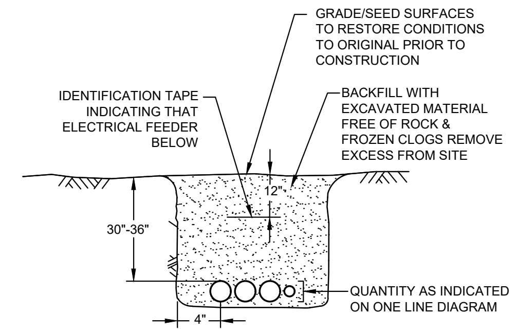
1 UTILITY TRENCH DETAIL E-501 SCALE: NONE
